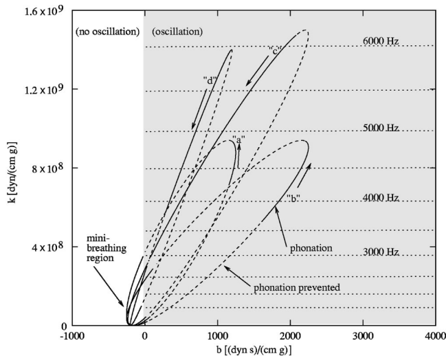
FIG. 7. Continuous path in parameter space leading to the simulated Chingolo's song of Fig. 1(b). Ellipse labeled "a" corresponds to the song's first syllable, and so on. Ellipses corresponding to consecutive syllables are smoothly matched in the mini-breathing region. Dotted line: large f_0 value (labia adducted, syrinx closed). Solid line: f_0=0 (syrinx open). As in Fig. 6, phonation occurs along the solid-line arcs in the oscillation region. Time parametrization is not illustrated; solid-line sections are traversed more slowly than dashed-line sections.
