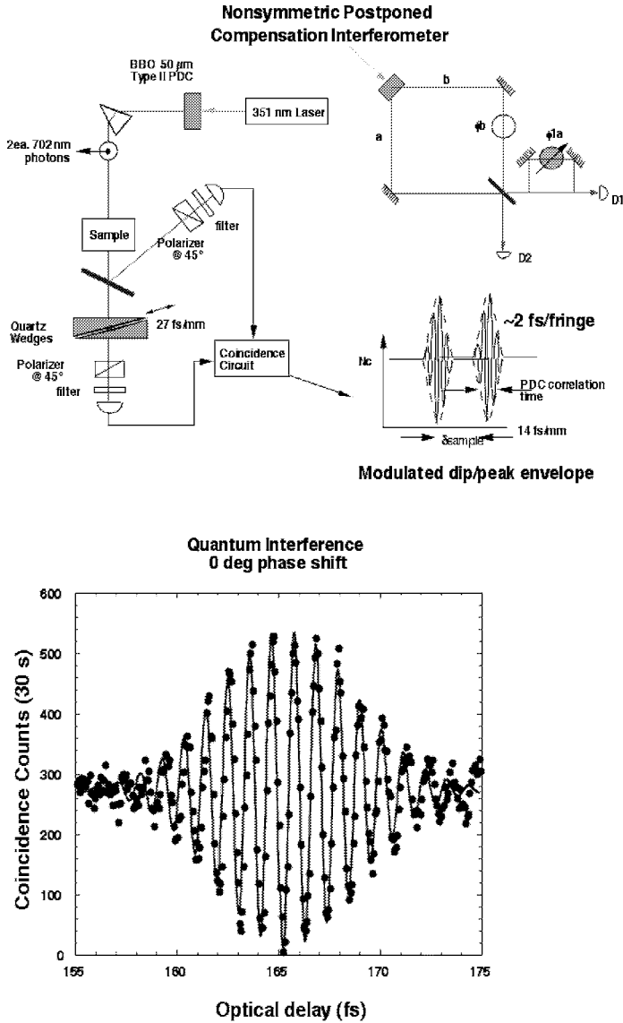
Figure 11. a) Schematic of a two-photon polarization interferometer with a postponed optical delay. This non-symmetric delay is introduced only in one arm after the beam splitter. b) Measurement of intensity correlations as a function of relative polarization delay d .
