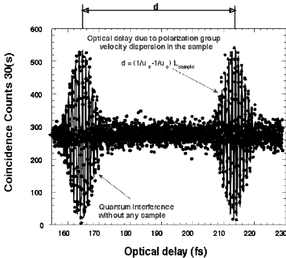
Figure 12. Measurement of the optical delay in the crystal quartz sample using a 50 \mu\text{m} nonlinear crystal. The horizontal scale is the time delay of the delay line located after the beamsplitter, BS.
