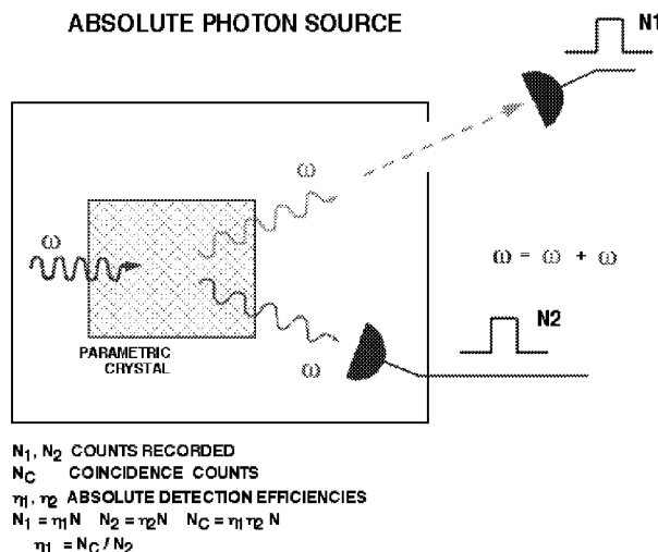
Figure 9. Principle of absolute calibration of quantum efficiency without using standards.
