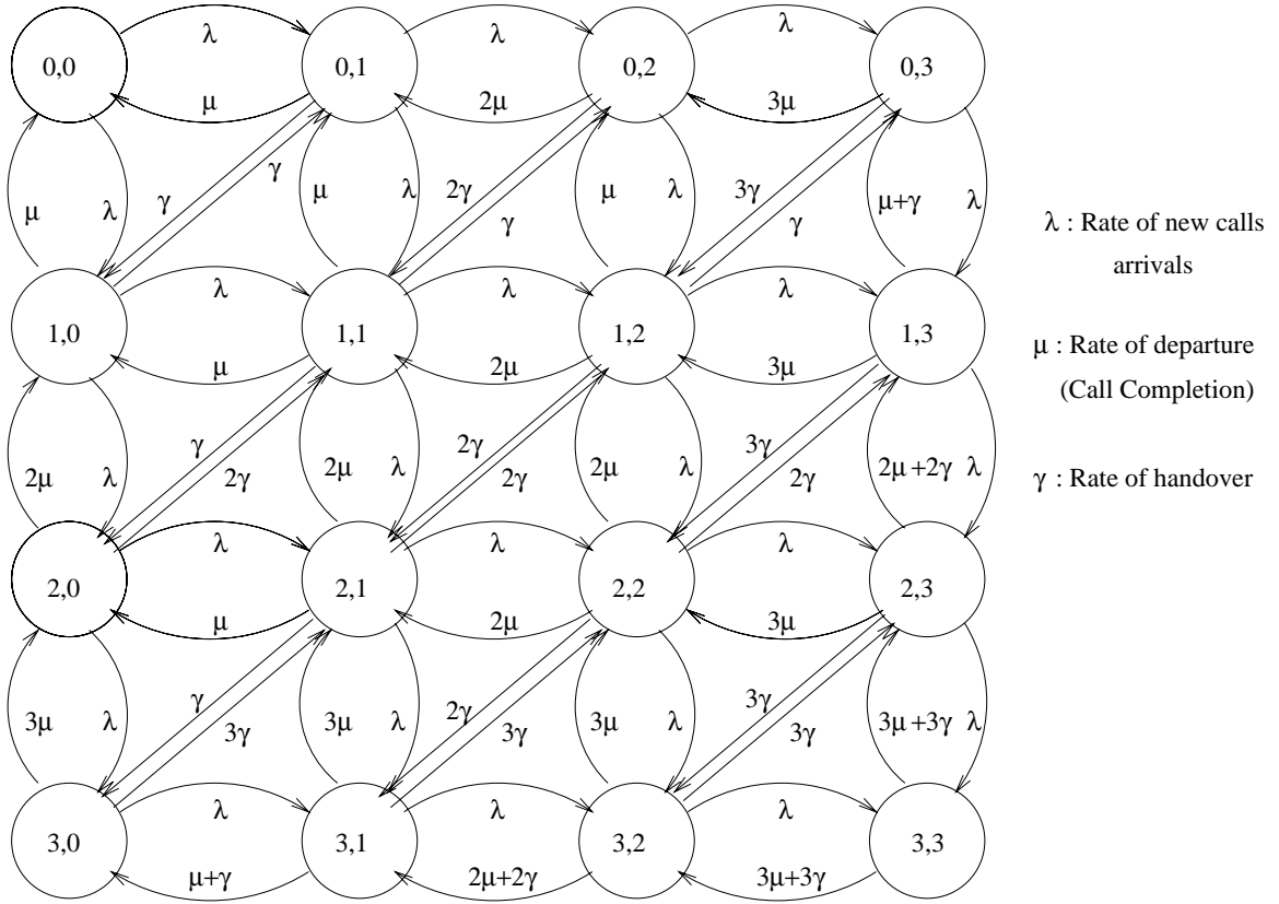
Figure 2: A Markov Chain describing 2 cells with 3 channels
