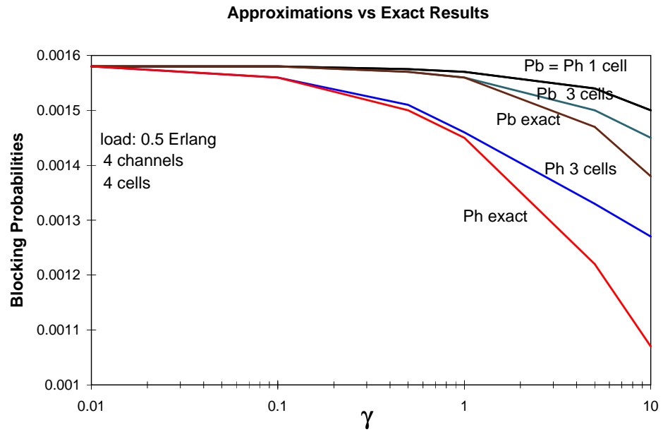
Figure 10: P_B and P_H vs \gamma : Comparison between the approximated and the exact results
