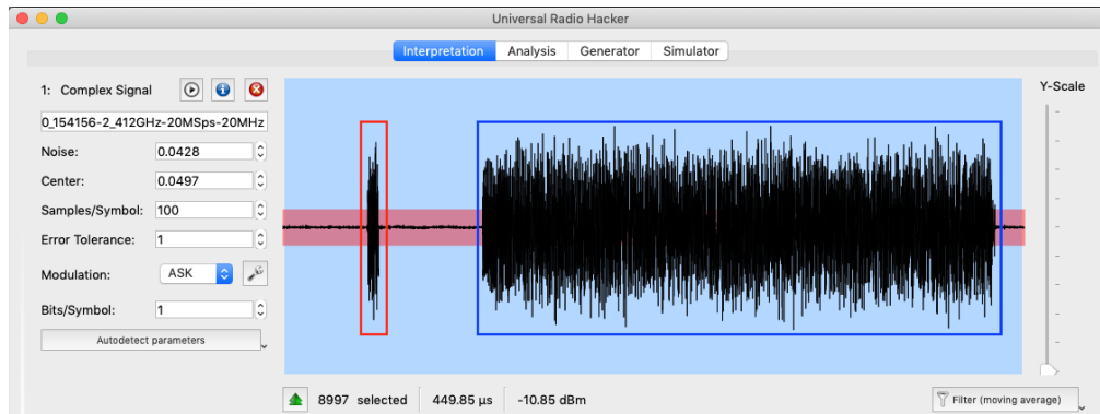
Figure 9: A signal recorded with urh [21] on an ADALM-PLUTO [1] shows the difference between a truncated preamble (left, delineated in red) and an actual packet (right, delineated in blue). The x -axis represents time, and the total duration of the signal captured here is 450 \mu s. When a legitimate packet follows a truncated preamble with such a short delay as shown in this scenario ( \approx 70 \mu s), a vulnerable device might not receive the message delineated in blue despite the absence of any collisions.
