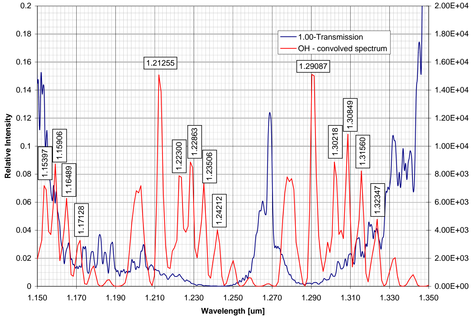
Night Sky Spectrum [J-Band, smoothed to 2.3nm resolution]
