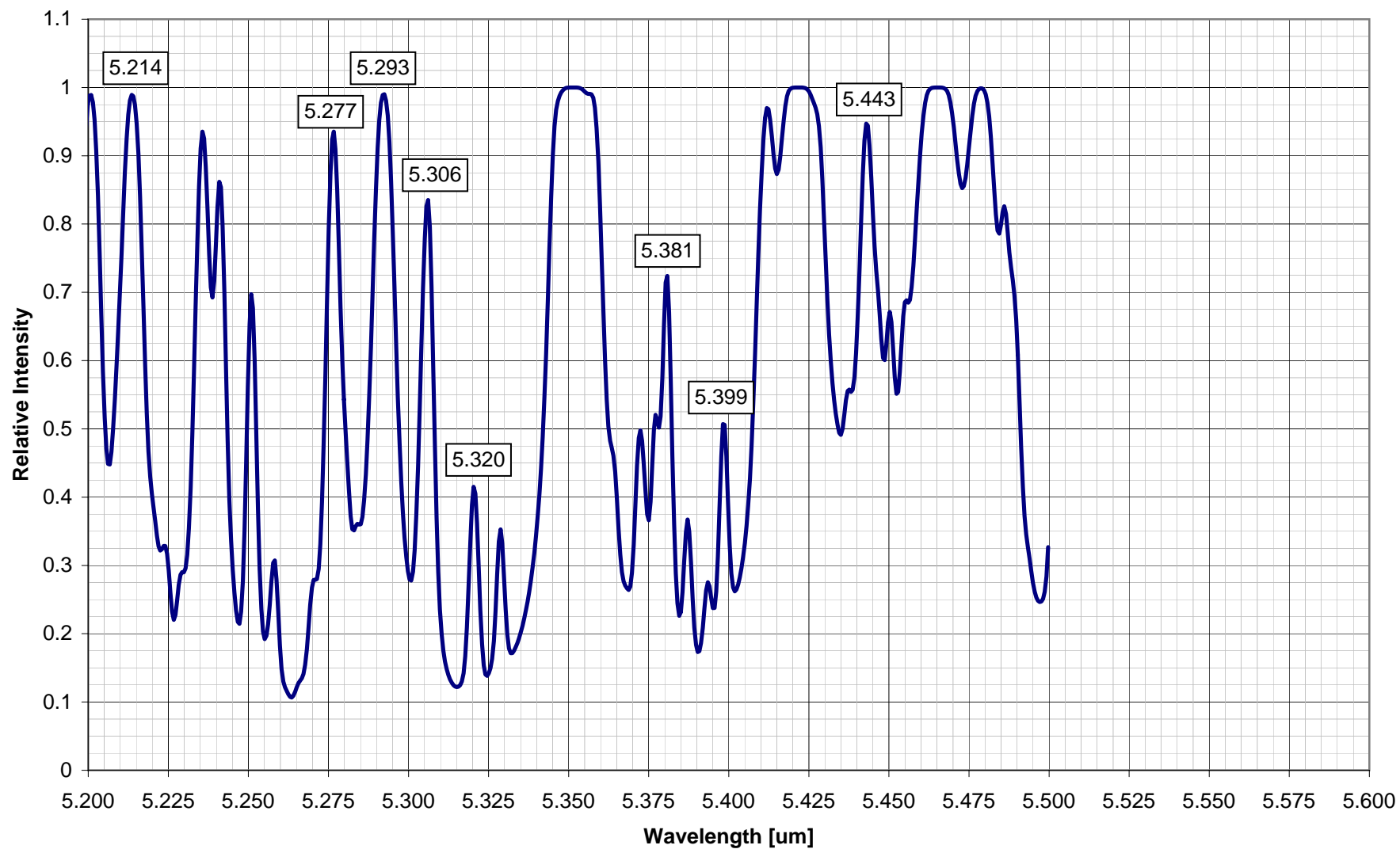
Night Sky Spectrum [5.2-5.6 um]
