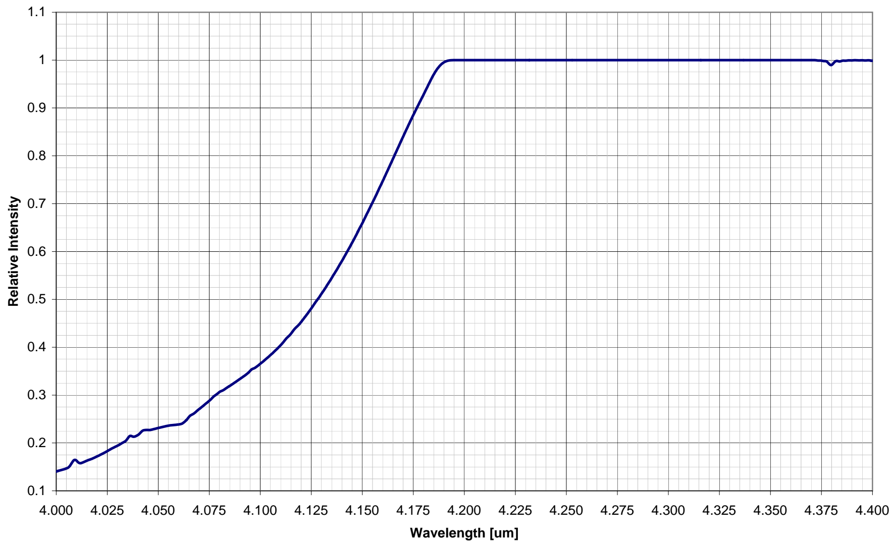
Night Sky Spectrum [4.0-4.4 um]
