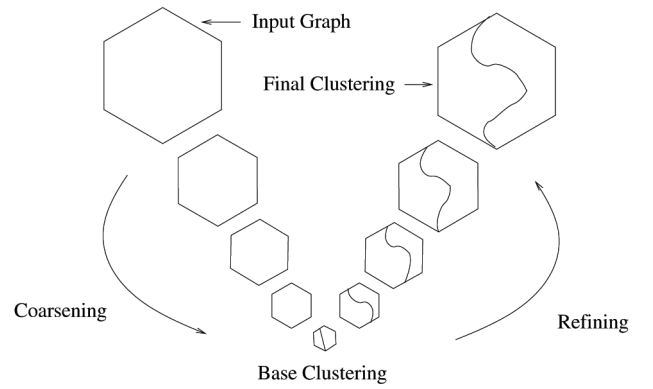
Fig. 1. Overview of the multilevel algorithm (for k = 2 ).
