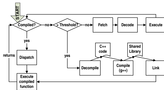
Figure 4. Dynamic-Compiled Simulator
