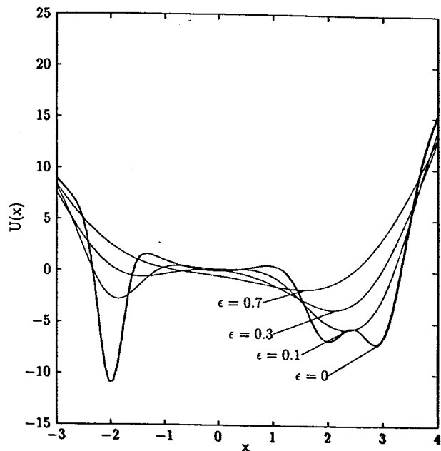
FIGURE 2. The potential function, eq. (28), is transformed using the Gaussian kernel. We show the transformed potentials for different values of the Gaussian width overlapped on the untransformed potential. The method fails by locating a local energy minimum.
