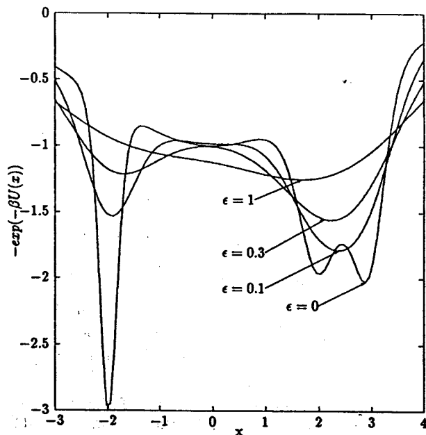
FIGURE 4. Gaussian smoothing is applied to find the minimum of M(U) = -\exp(-\beta U(x)) using \beta = 1/10 in order to find the global minimum of the potential function, eq. (28). The method fails by locating a local energy minimum.
