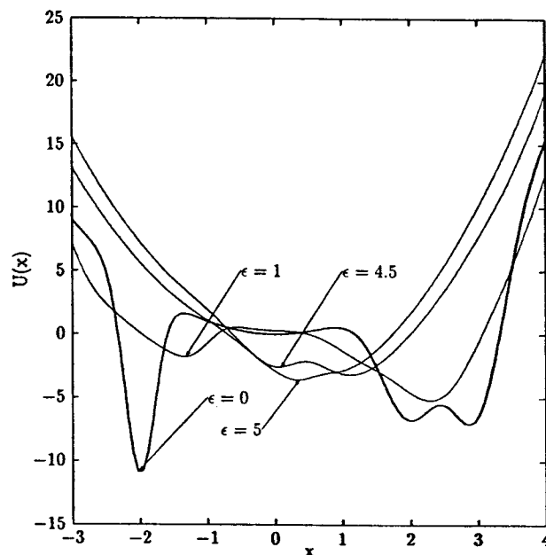
FIGURE 1. The method of bad derivatives is used to smooth the potential function, eq. (28). The transformed potential is overlapped on the untransformed potential for different values of parameter \epsilon . The arrows also indicate the position of the minimum traced by local minimization for each of the curves. By tracing back the position of the minimum the method of bad derivatives succeeds in locating the global minimum of the original potential.
