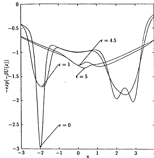
FIGURE 3. The method of bad derivatives applied to find the minimum of M(U) = -\exp(-\beta U(x)) using \beta = 1/10 in order to find the global minimum of the potential function, eq. (28). The position of the global minimum is found correctly.
