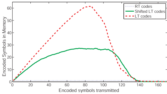
Fig. 2. Memory usage at the decoder as a function of the number of transmitted symbols.
