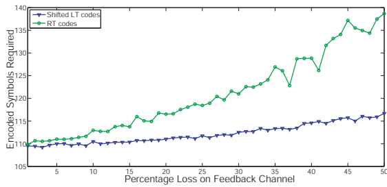
Fig. 6. The number of encoded symbols needed to decode 100 input symbols, as a function of the feedback channel loss rate. The forward channel loss rate is fixed at 5%.
