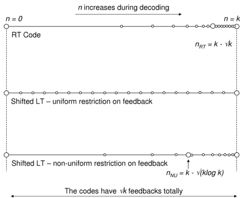
Fig. 1. Feedback strategies for uniform and non-uniform restrictions on Shifted LT and RT codes. Each circle qualitatively corresponds to a situation in which the current value of n is fed back to the encoder.
