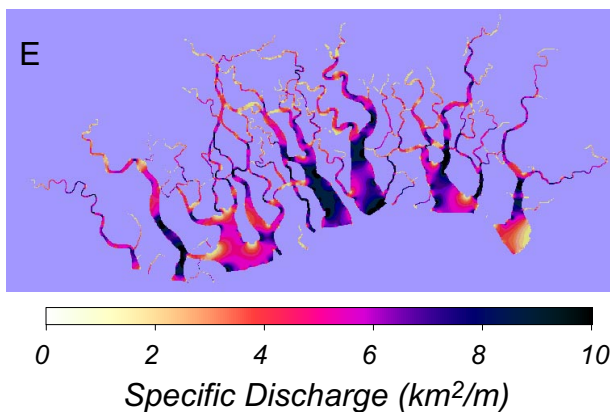
Fig. 1. Morphological analysis of tidal deltas. (A) LANDSAT image of the Sunderbans, in the Ganges Delta, Bangladesh (courtesy NASA World Wind). (B) LANDSAT image of the Kikori delta, Papua New Guinea. (C) Tidal channel
