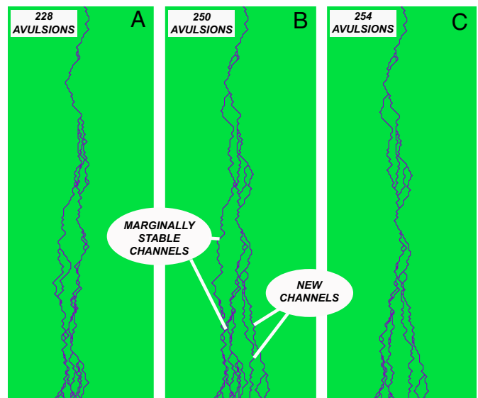
Fig. 2. Simulation of tidal delta evolution. At each time step a new avulsion is created within the delta. All of the channels with a specific tidal discharge below the threshold value are abandoned and removed from the delta. Delta after 228 avulsions (A), after 250 avulsions (B), and after 254 avulsions (C). The delta extends in the lower right area between avulsion 228 and 250, but this extension destabilizes the upper left part of the delta that collapses at avulsion 254.
