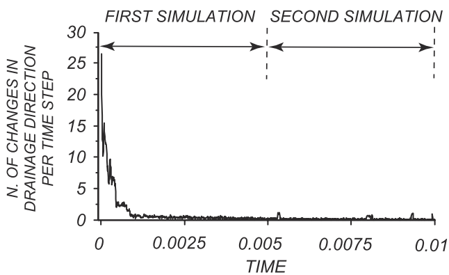
Figure 3. Number of nodes changing drainage direction in each time step. The data are averaged over 20 steps to eliminate short-term fluctuations.
