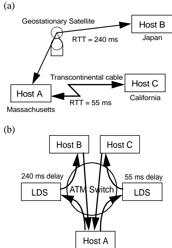
Figure 2: (a) A network configuration example; and (b) simulated lab configuration using two instances of LDS and an ATM switch. The VCI/VPI values of ATM cells will pass through the LDS unchanged.
