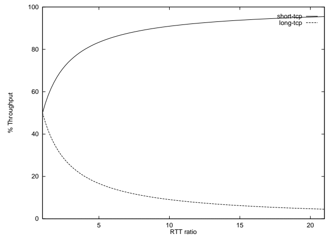
Figure 6: Predicted Throughput vs. RTT Ratio.
