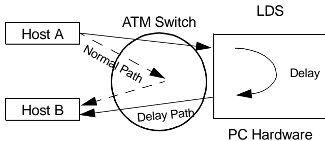
Figure 1: A typical LDS configuration for experimental use. The solid arrows indicate the delayed path through the LDS; the dashed line shows the non-delayed path.
