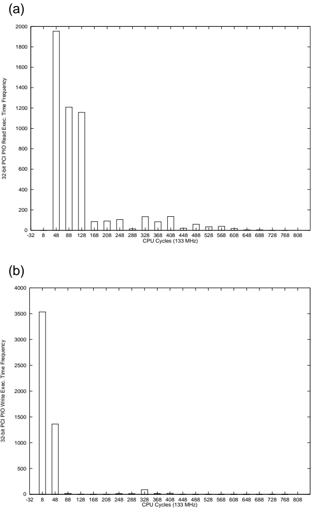
Figure 3: (a) Histogram of 32-bit programmed I/O PC read times; (b) Histogram of 32-bit programmed I/O PCI write times. All are for 354-cell buffers.
