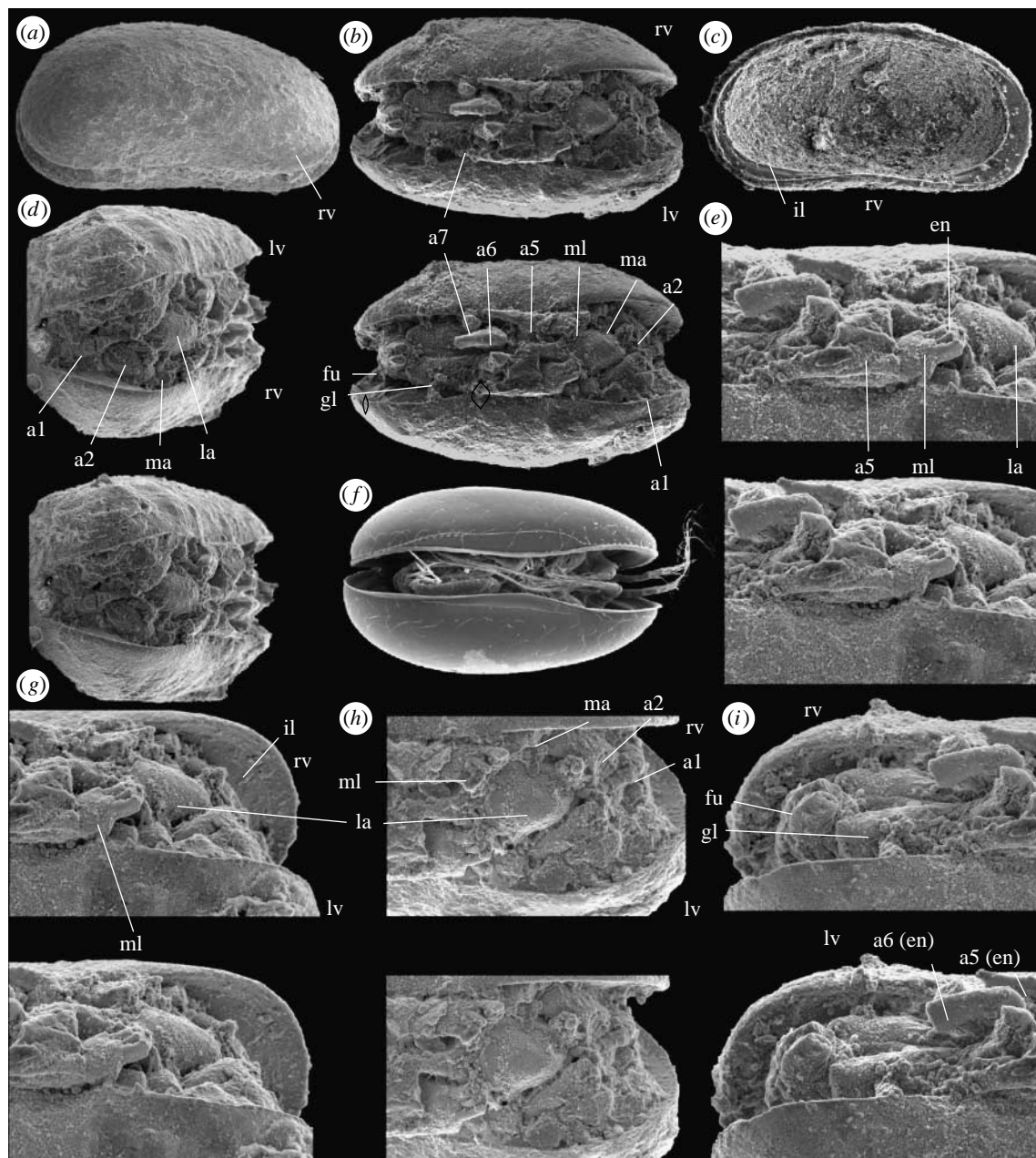
Figure 1. ( a–e, g–i ) Scanning electron micrographs of Lacalgida avia : ( a ) right lateral view of carapace, OUMNH NS.2, x82.5; ( b, d, e, g–i ) holotype with near complete complement of appendages and soft anatomy, OUMNH NS.1; ( b ) ventral view (stereo pair), x84; ( d ) anterior view (stereo pair) showing the first and second antenna (visible on the right side), mandible and labrum, x100; ( e ) oblique ventral view of labrum, mandible and second maxilla (stereo pair), the basipod of the latter with three terminal endites, x160; ( g ) oblique ventral view of anterior (stereo pair) with first and second antennae visible on the right side, x160; ( i ) oblique ventral view of posterior (stereo pair) with endopods of sixth and seventh walking appendages, genital lobes and furcal rami, x160. ( c ) right valve, internal lateral view, OUMNH NS.3, x94; ( f ) modern female specimen of the candonid ostracod Physocypria nipponica Okubo 1990, ventral view, x81. This specimen, from the southern basin of Lake Biwa, Shiga Prefecture, Japan, is used for a simple comparison of soft anatomy and no close relationship to L. avia is inferred (Abbreviations: a1, first antenna; a2, second antenna; a5–a7, fifth to seventh appendages, a5 (en), a6 (en), endopods; ma, mandible; ml, first maxilla; la, labrum; fu, furcal ramus; rv, right valve; lv, left valve; il, inner lamella; gl, genital lobe; en, endite.).
