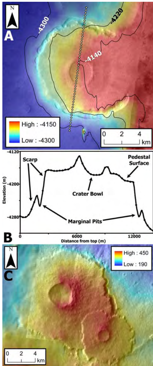
Figure 3. (a) A pedestal crater with marginal pits that have coalesced to form a moat-like structure (subscene of THEMIS image V10457014; 60.2^{\circ}\text{N} , 102.5^{\circ}\text{E} ). (b) Altimetry profile across the pedestal crater in Figure 3a. (c) One pedestal partially draped over another (THEMIS mosaic; 61.3^{\circ}\text{S} , 71.2^{\circ}\text{E} ). The larger pedestal has developed marginal pits, one of which is truncated by the smaller pedestal. This superposition relationship suggests that pedestals did not all form from the same ice-rich mantle; rather they formed during multiple periods of mantle emplacement and removal.
