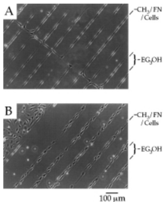
FIG. 7. Optical micrograph of cells attached to patterned SAMs of alkanethiolates on silver having lines with sizes of 10 \mu\text{m} (A) and 30 \mu\text{m} (B) and separated by inert regions 120 \mu\text{m} in width. The cells were plated and maintained in defined medium. The scale bar applies to both images.
