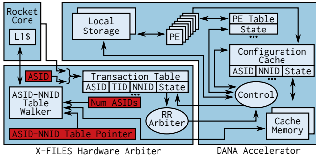
Fig. 2. The X-FILES/DANA hardware architecture. Neural network transactions are managed by a hardware arbiter and executed on a backend accelerator.
