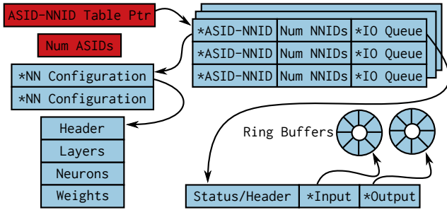
Fig. 1. An ASID-NNID Table for dereferencing NN configurations
