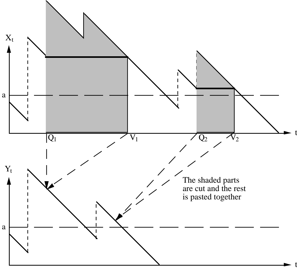
Figure 2: Construction of Y_t based on X_t for the M/GI/1 queue with with balking
