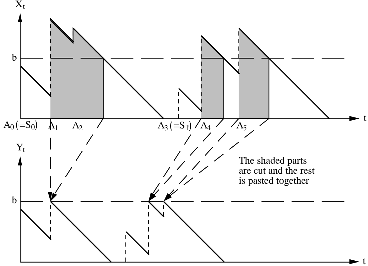
Figure 1: Construction of Y_t based on X_t for the M/GI/1 queue with bounded workload process
