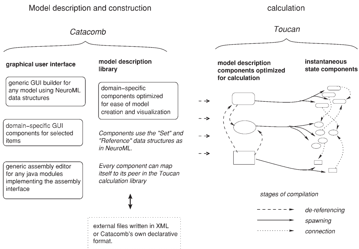
Fig. 3. Catacomb2 system architecture is divided into two distinct parts: Catacomb itself, which is concerned with the description, construction and visualization of models of biological systems; and Toucan, a numerical calculation package designed for memory-efficient calculation of model behavior. Toucan is a free-standing package which can be used entirely independently of the model description tools. Catacomb comprises model description components, a generic user interface system which can construct any model consistent with the data structures employed, and as large set of domain-specific user interface components for the exploration of certain types of models. The only part of the whole system which is persistent (can be saved to files and restored) is the description of the active model.
