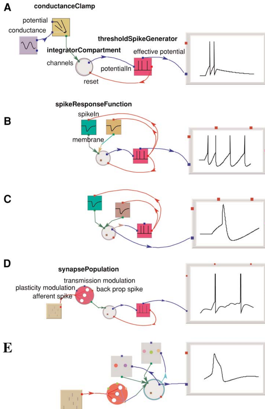
Fig. 1. Component-based single cell models. The components on the left are used for stimulation, either by imposing a transient conductance change on the membrane ( A , B , and C ) or by sending a train of events to a population of synapses ( D and E ). The right-most component shows the membrane potential of the cell. All figures are generated directly from the software and appear much as they do through the user interface. A . Simple integrate-and-fire cell with a leaky integrator compartment and a spike generator which fires an event whenever the cell exceeds a threshold. The spike generator reads the potential of the cell and causes the potential to be reset when it fires an event (link going back to the “reset” port on the integrator compartment). B . As case A , but with the addition of two spike response functions that are triggered by events from
