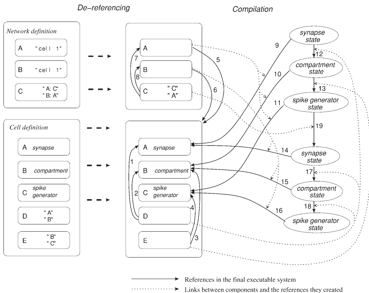
Fig. 4. Stages in the preparation of an executable Toucan model instance. Solid arrows show direct references in the final data structure; dotted ones indicate which component is responsible for creating each reference. Numbers show the order in which references are created. There is a network of two cells of the same type ( A and B at the top) with a single connection between them ( C ). The cell model has three components with two connections. First the references by name are looked up, giving the solid arrows in the middle section. Then the network creates an executable instance. The first cell reference calls the cell description to create a state instance. Each of the first three components in the cell description spawns a state instance; the last two make connections between them. This process is repeated when the second cell reference in the network calls for an executable instance. Finally the third component of the network, the connection between the two cells, finds and connects the appropriate subcomponents of the two cell instances.
