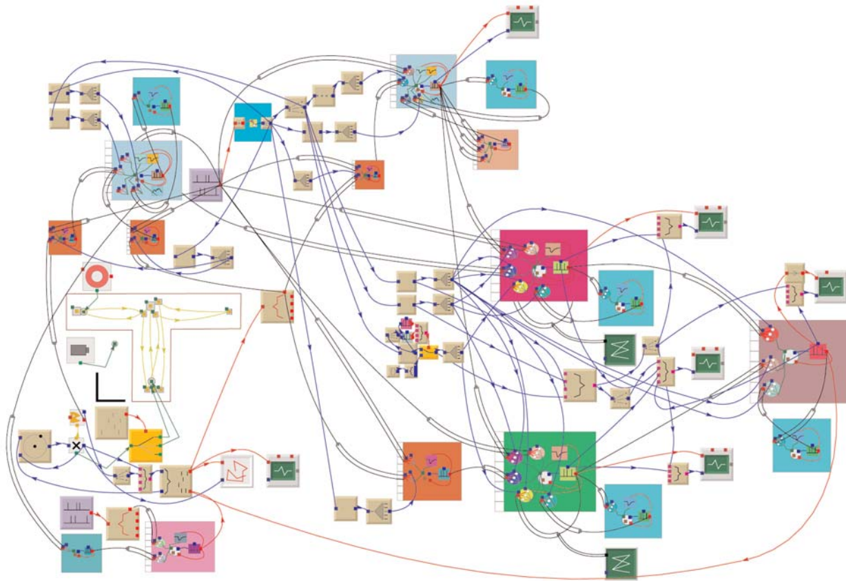
Fig. 6. T-maze, virtual rat and network as it appears in Catacomb2. The symbols correspond to the items in Tables 3–7. Larger boxes with a ladder down the left hand side are populations of cells, and double lines represent 1-1 or all-all projection patterns between populations. [CFO]
