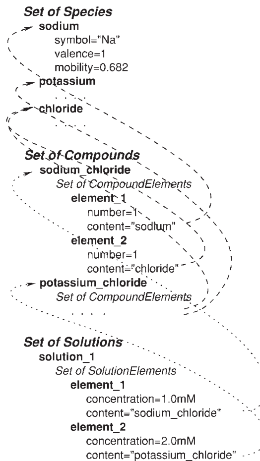
Fig. 2. Set and reference structure for describing aqueous solutions. Slanting text indicates sets, bold normal text model components, and plain text fields and their values. Parts of the description have been omitted as indicated by rows of dots. Each specie is defined only once, in a top-level set of species. Likewise compounds and solutions are kept in top level sets. Each compound needs to refer to the species it contains, but with each reference it also needs to specify the number of occurrences. Therefore each compound has a local set of CompoundElement objects which are not visible elsewhere. Each element contains a number and a reference to the corresponding specie (dashed lines). Similarly, solutions contain a local set of objects to combine the concentration of a compound with a reference to its content (dotted lines).
