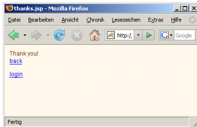
Figure 16: thanks.jsp
