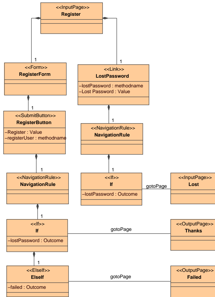
Figure 14: Modeling of Pageflow for the Register Web page
