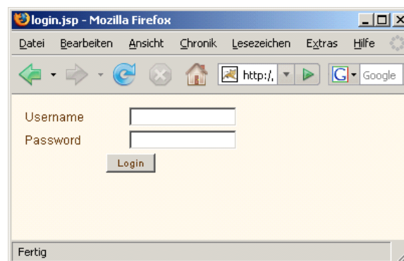
Figure 19: login.jsp
