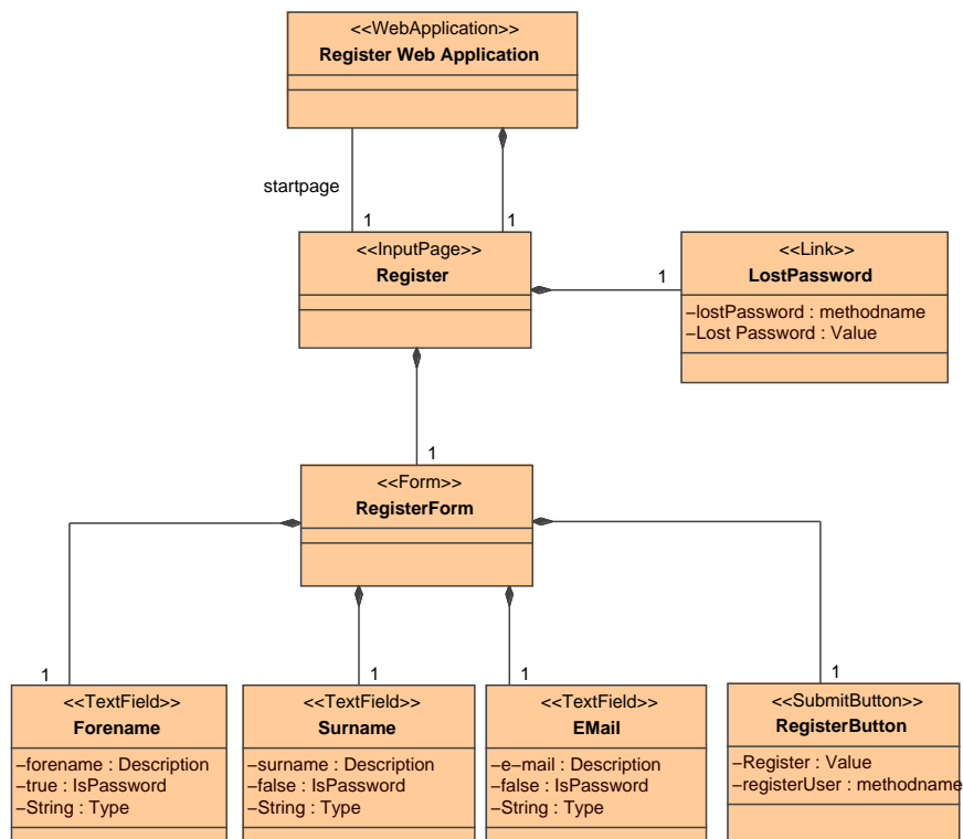
Figure 12: Model of a Web page
