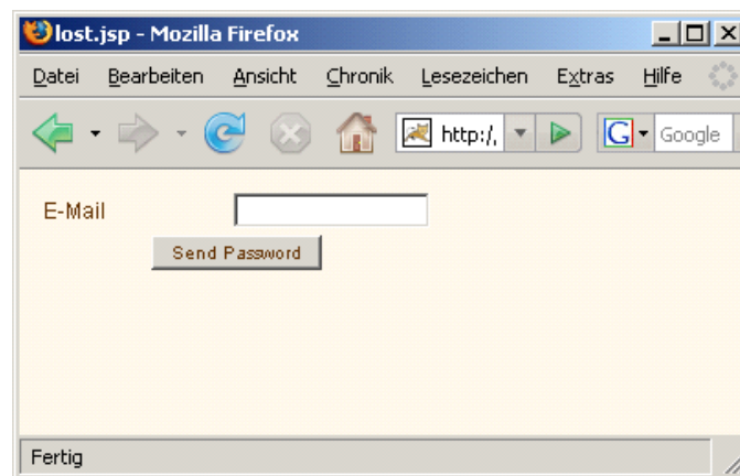
Figure 18: lost.jsp
