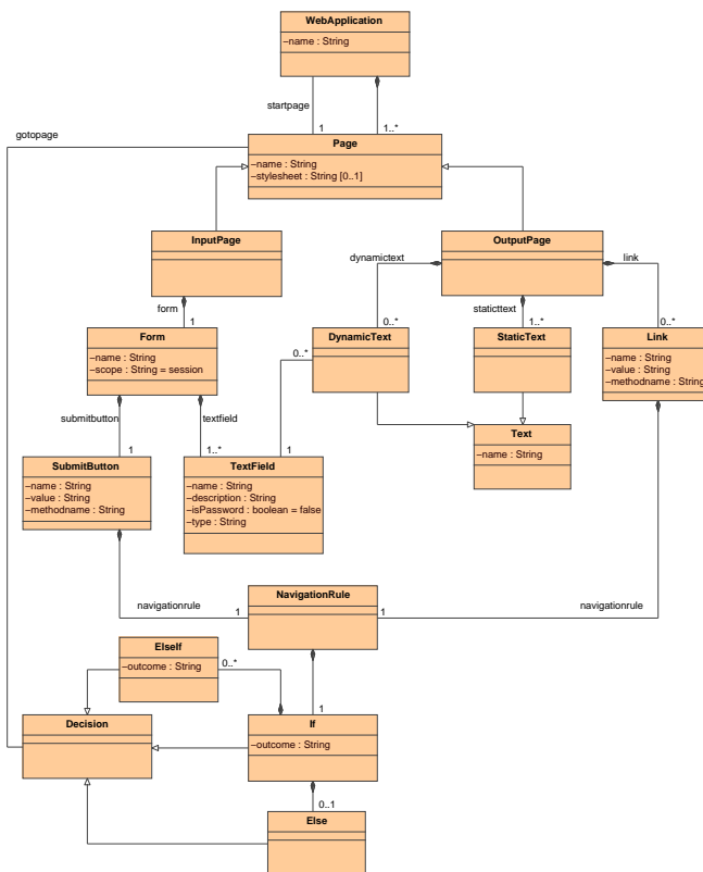
Figure 6: Metamodel
