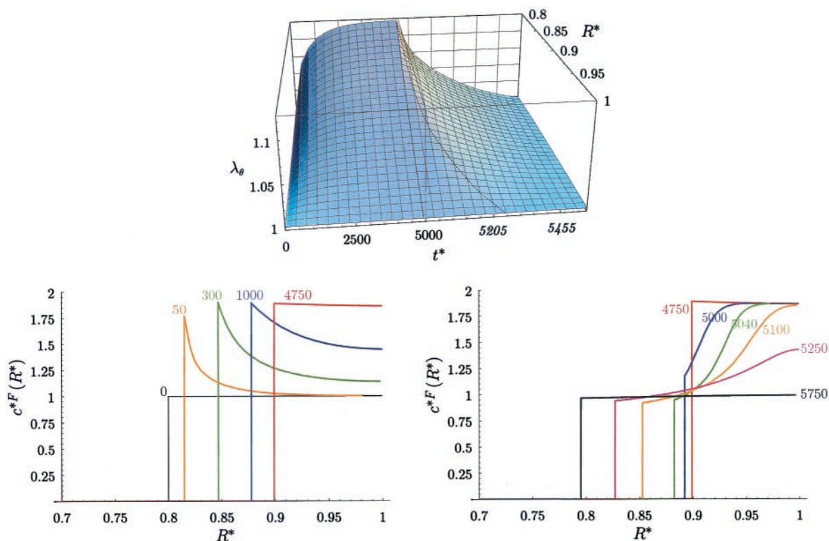
FIGURE 3 Three-dimensional plot (top) of the displacement field over space and time for the same parameter values as in Fig. 2 except that M = 8 . Note that the time scale changes at t = 5,000 , from 500 units per minor axis division to 41 units per division, and this is demarcated by the straight dashed line. Thus compression takes about ten times longer than recovery for this value of M . The dashed curve corresponds to the location of a front where there is a sharp change in the slope of \lambda_\theta . Instantaneous glycocalyx concentration distributions for different times (as indicated beside each curve) during compression (bottom left) and recovery (bottom right). The concentration front propagating through the glycocalyx during recovery of the matrix is evident in these distributions. Units of time are as in Fig. 2.
