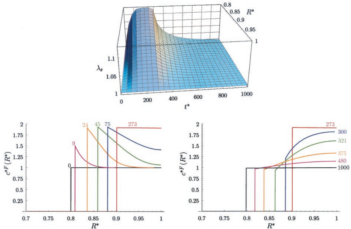
FIGURE 2 Three-dimensional plot (top) of the displacement field over space and time for \mathcal{F} = 10^{-7} , \xi_0 = 0.01 , and M = 0 . Glycocalyx concentration over space for different times (as indicated beside each curve) during compression (bottom left) and recovery (bottom right). The compressing load was applied in a time \tau_{\text{load}} = 10 , which is more than 20 times faster than either the compression or recovery times. All times are in units of \sqrt{\mathcal{F}}\tau_c = R_0^2/(k_0 k_B T c_0^+) = 1.79 \times 10^{-3} s for R_0 = 2.5 \mu\text{m} , k_0 = 10^{-11} \text{cm}^4(\text{dyn}\cdot\text{s})^{-1} , and c_0^+ = 0.14 M). Equation 53 reveals that, if \xi_0 \ll 1 , the local glycocalyx concentration, c^{*F}(R^*, t^*) , is directly proportional to the local voltage potential, V^*(R^*, t^*) , and thus the instantaneous concentration distributions shown in the bottom two panels correspond to the instantaneous voltage distributions if the vertical axis is scaled by the factor 1/2k_B T \xi_0/q = 0.129 mV, i.e., at equilibrium, the glycocalyx is 0.129 mV above the lumen if \xi_0 = 0.01 .
