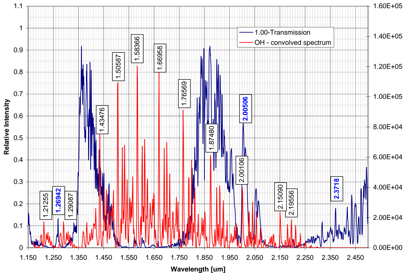
Night Sky Spectrum [JHK-Band, smoothed to 2.94nm resolution]
