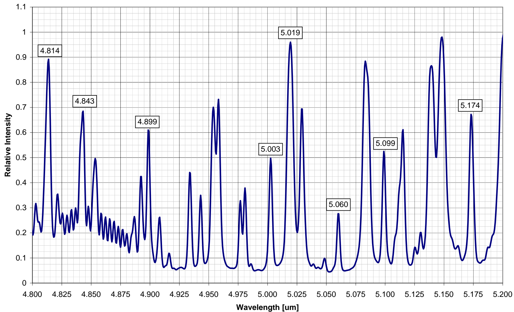
Night Sky Spectrum [4.8-5.2 um]
