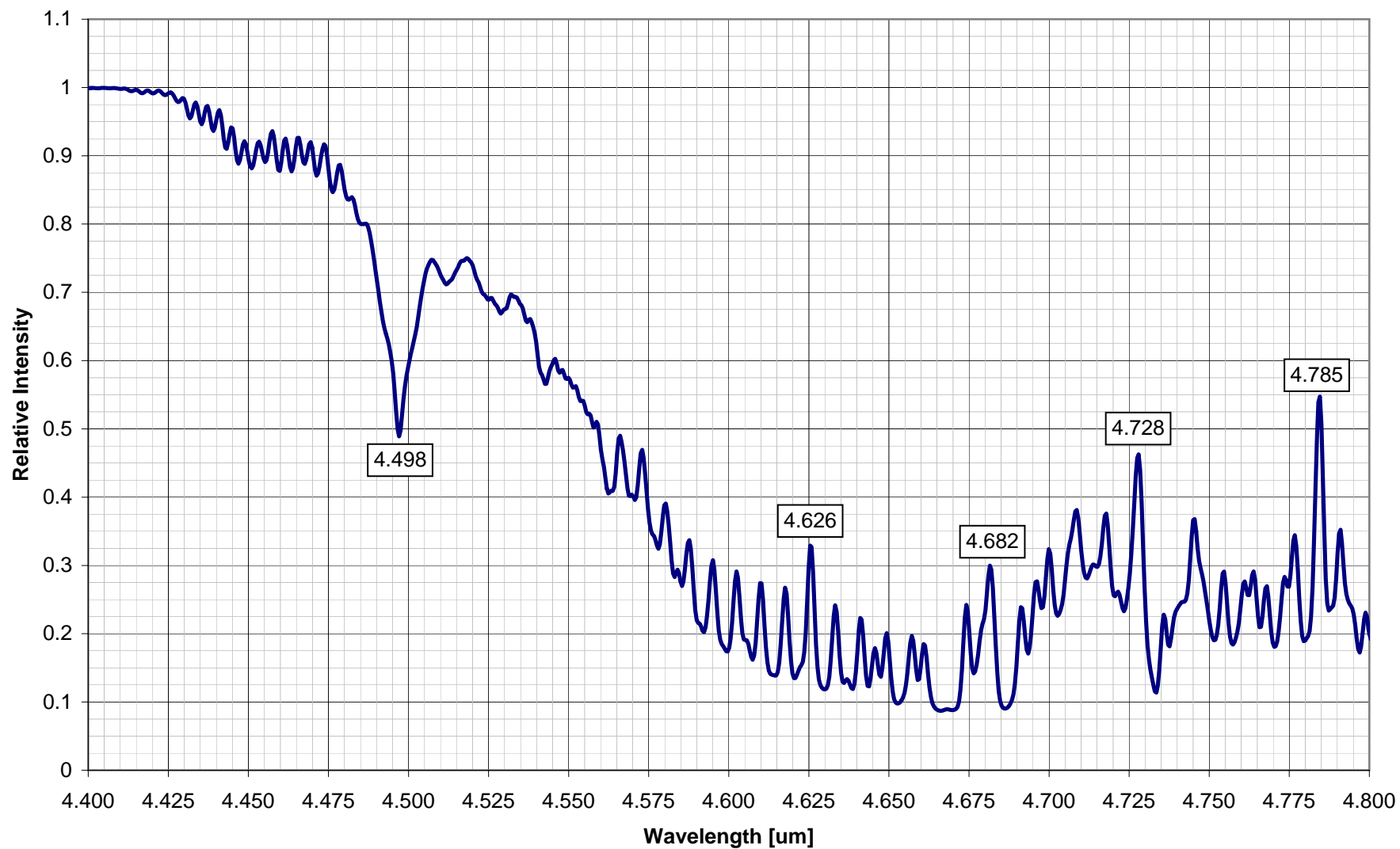
Night Sky Spectrum [4.4-4.8 um]
