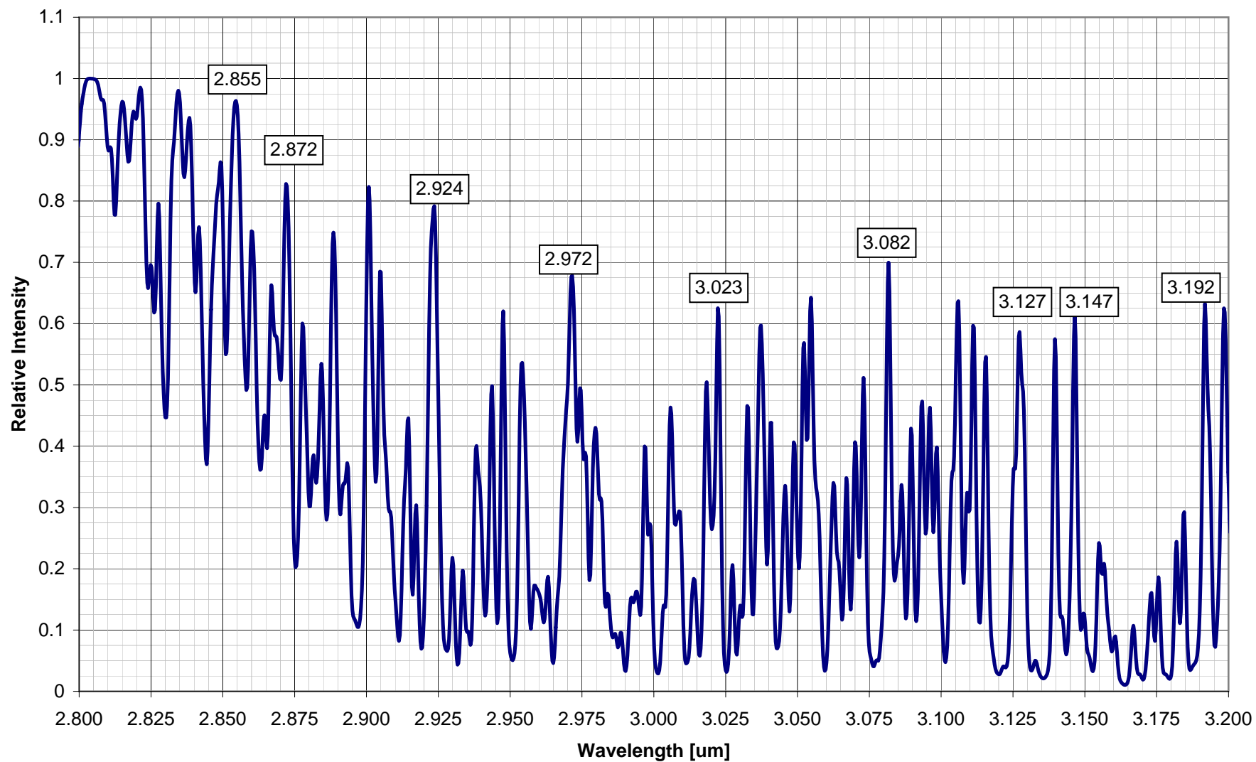
Night Sky Spectrum [2.8-3.2 um]
