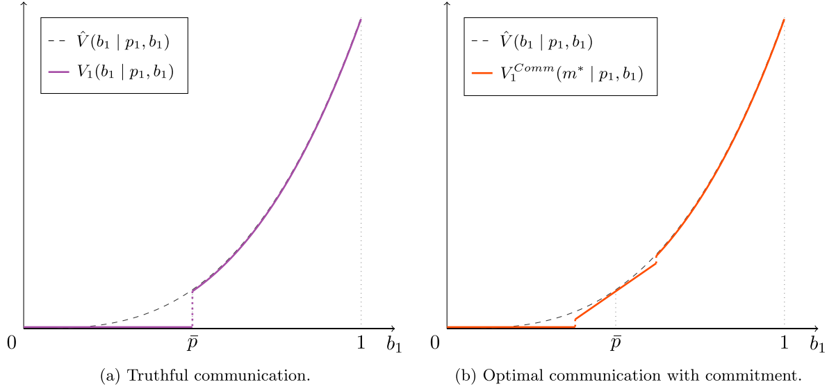
Fig. 2. C_1 's continuation value given different communication strategies.
