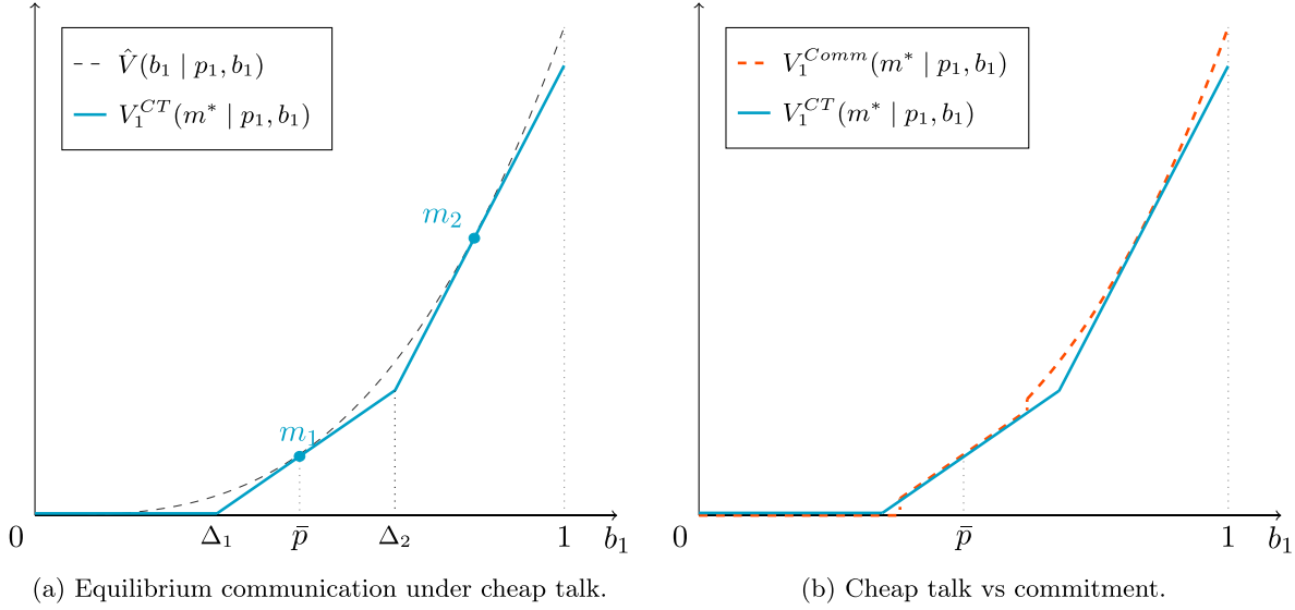
Fig. 3. C_1 's continuation value with cheap talk.
