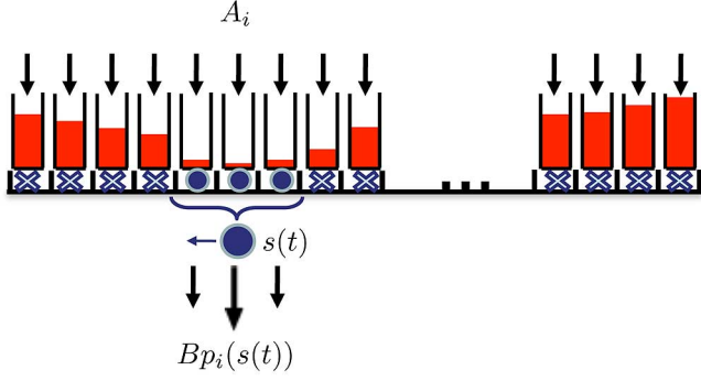
Fig. 1. Queueing system analog of the persistent monitoring problem.
