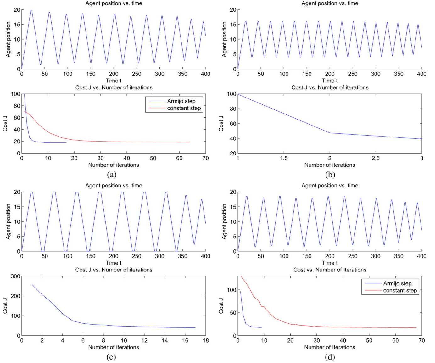
Fig. 3. One agent example. L = 20 , T = 400 . For each example, top plot: optimal trajectory; bottom plot: J versus iterations. (a) a = 0 , b = 20 . A_i = 0.1 , i = 0, \dots, 20 , J^* = 17.77 . (b) a = 4 , b = 16 . A_i = 0.1 , i = 0, \dots, 20 . J^* = 39.14 . (c) a = 0 , b = 20 . A_0 = A_{20} = 0.5 , A_i = 0.1 , i = 1, \dots, 19 . J^* = 39.30 . (d) a = 0 , b = 20 . A_i(\Delta t_i) \sim U(0.0075, 0.125) , \Delta t_i \sim 0.1e^{-0.1t} . J^* = 17.54 .
