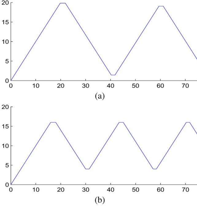
Fig. 4. Magnified trajectory for sub-figure (a) and (b) in Fig. 3, t \in [0, 75] .
