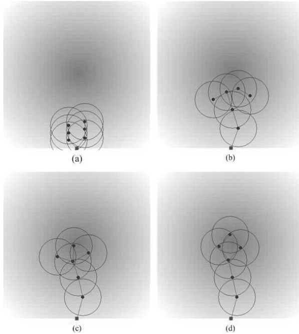
Figure 12: Sensor node deployment with communication cost consideration
