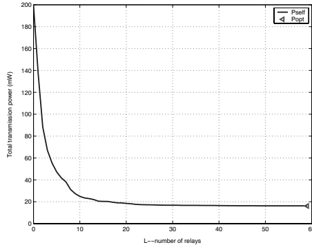
Figure 5: Incremental self-deployment algorithm performance as a function of nodes deployed
