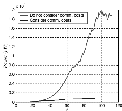
Figure 14: Comparison of communication costs
