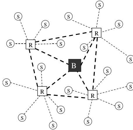
Figure 1: A 3-layer sensor network structure
