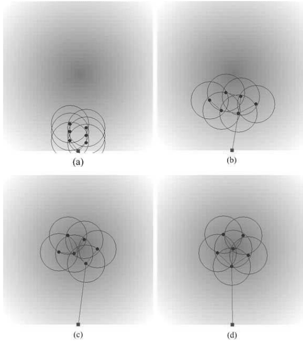
Figure 11: Sensor node deployment without communication cost consideration
