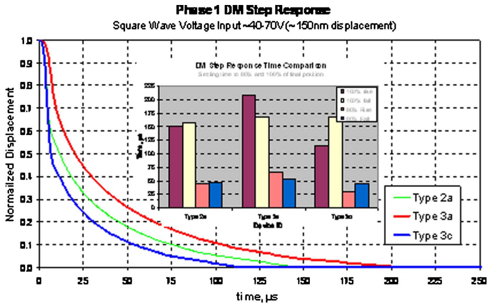
Fig. 14 Normalized dynamic response of each of the three DM design types to a square wave input of ~30 V P-P, corresponding to a displacement of ~150 nm. Each of the three devices settles within 200 \mu s in response to the voltage step input.
