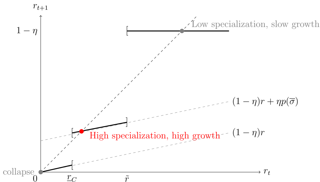
Figure 2: The Hopeful Case ( \underline{r}_C < r^* < \hat{r} ): High Growth
